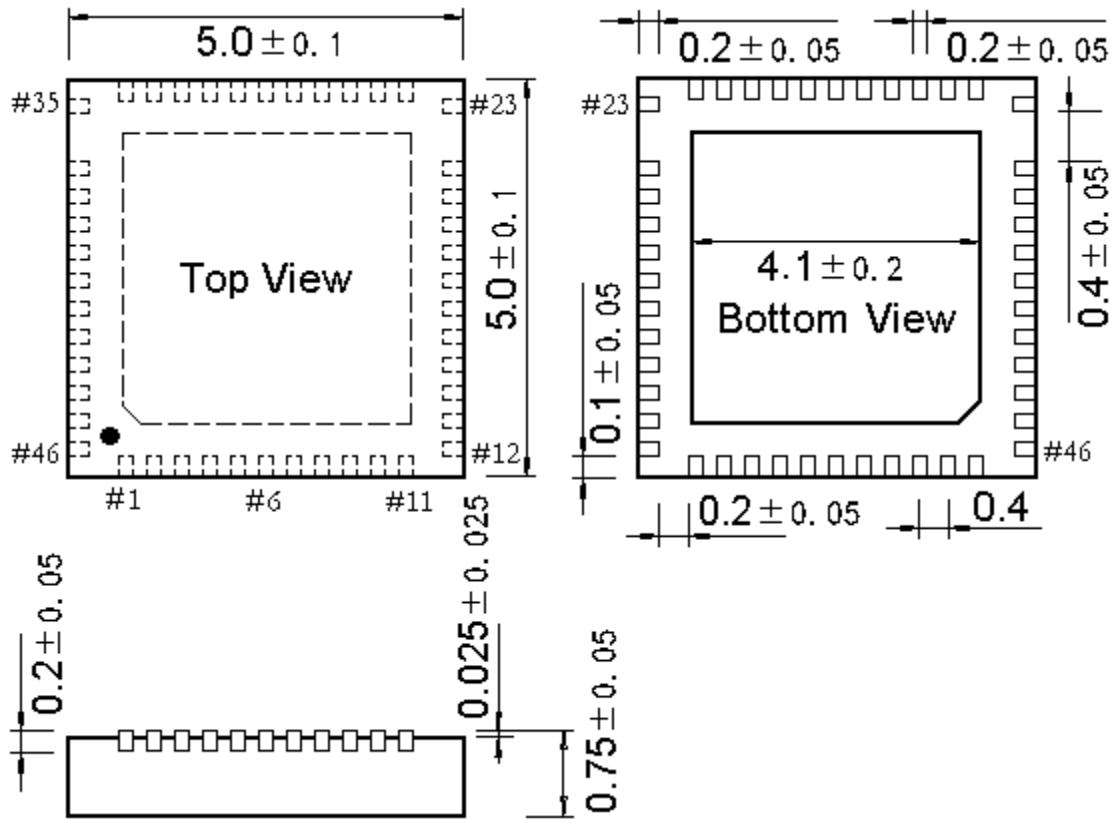
QFN46C5 (QFN46C-5*5*0.75-0.4)
