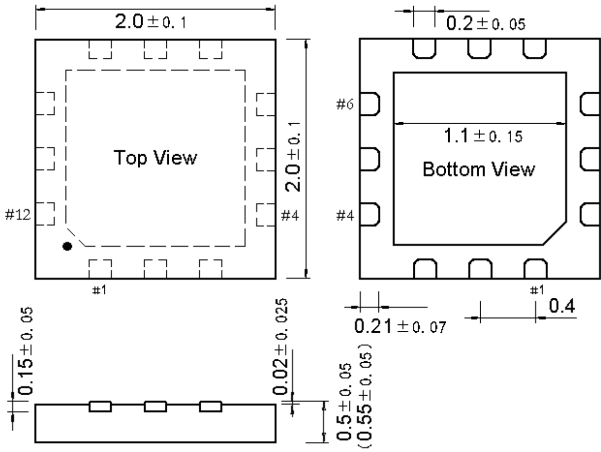
QFN12 (QFN12-2*2*0.5-0.4)
