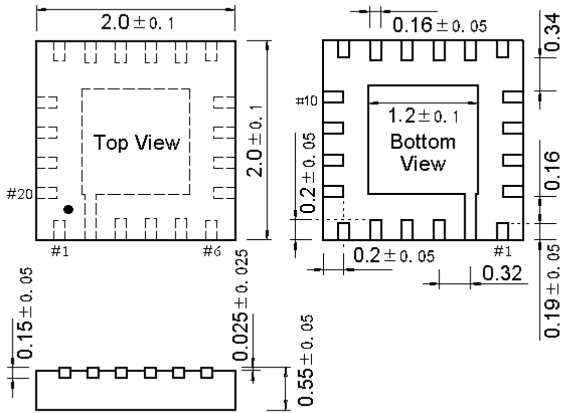
QFN20C2 (QFN20C-2*2*0.55-0.32)
