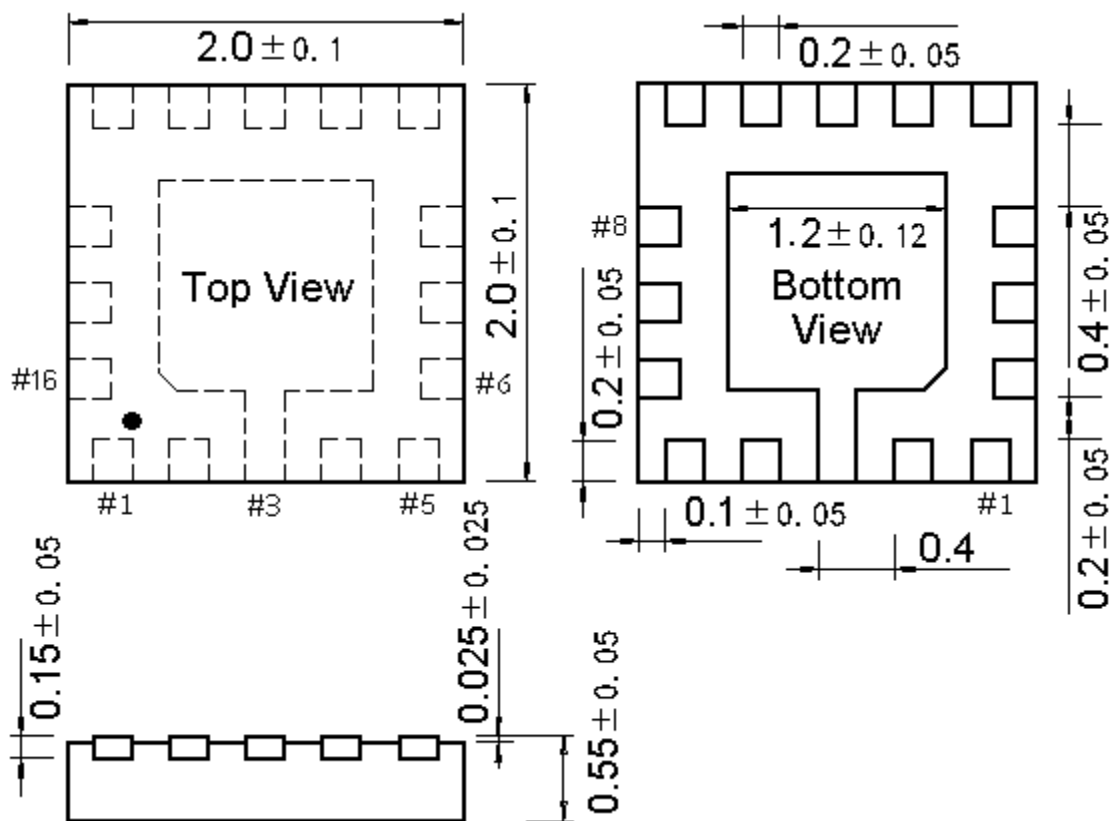
QFN16C2 (QFN16C-2*2*0.55-0.4)
