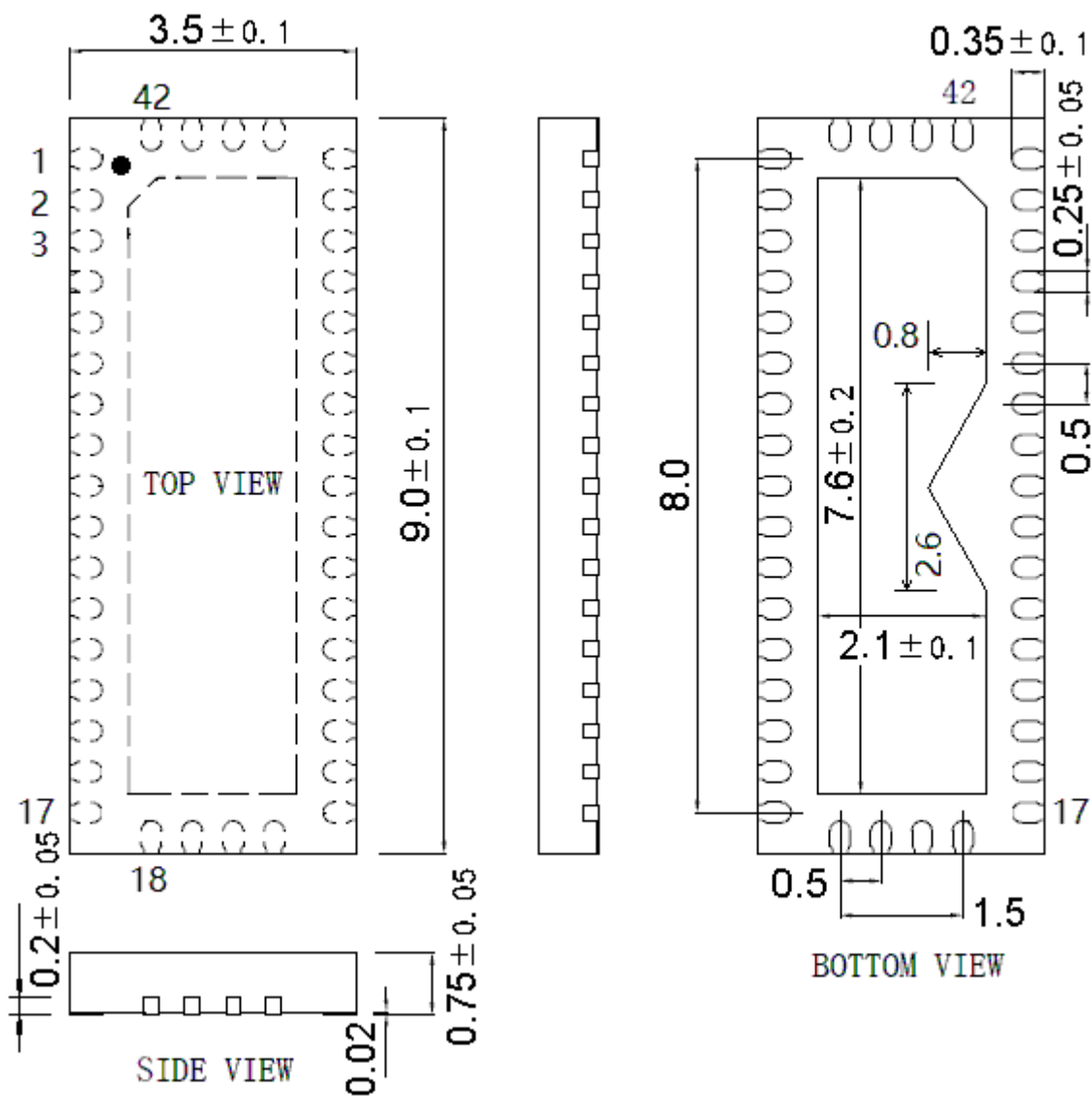
QFN42C35X9 (QFN42C-3.5*9*0.75-0.5)
