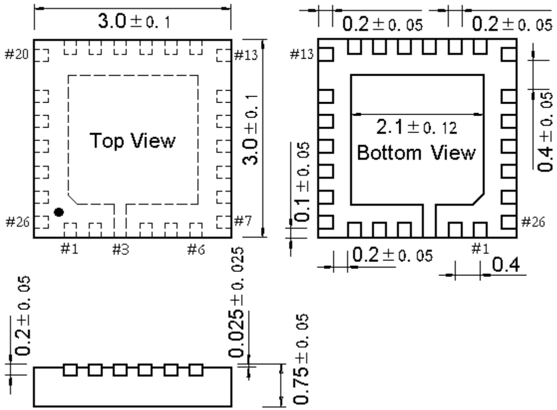
QFN26C3 (QFN26C-3*3*0.75-0.4)
